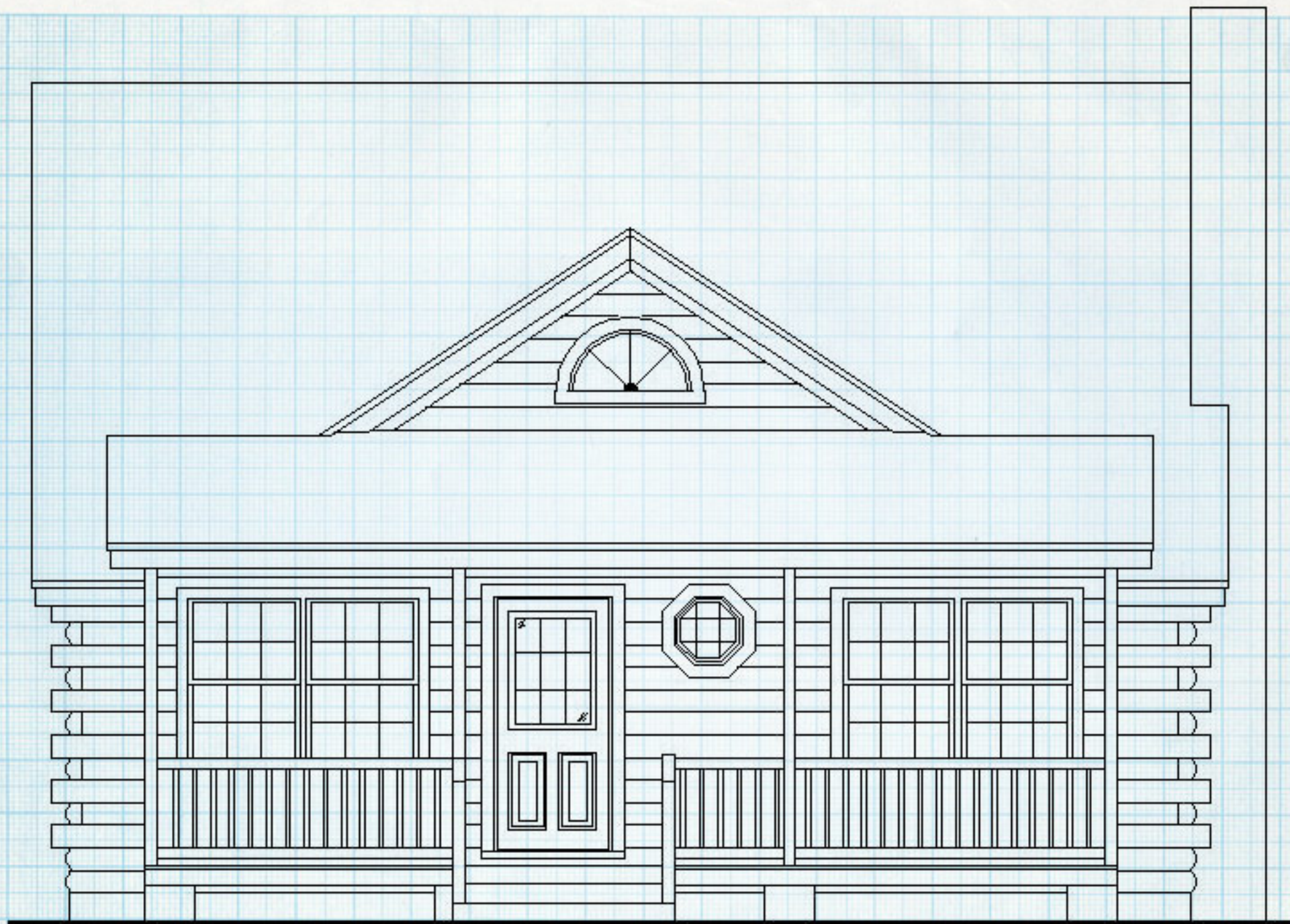
FRONT ELEVATION
