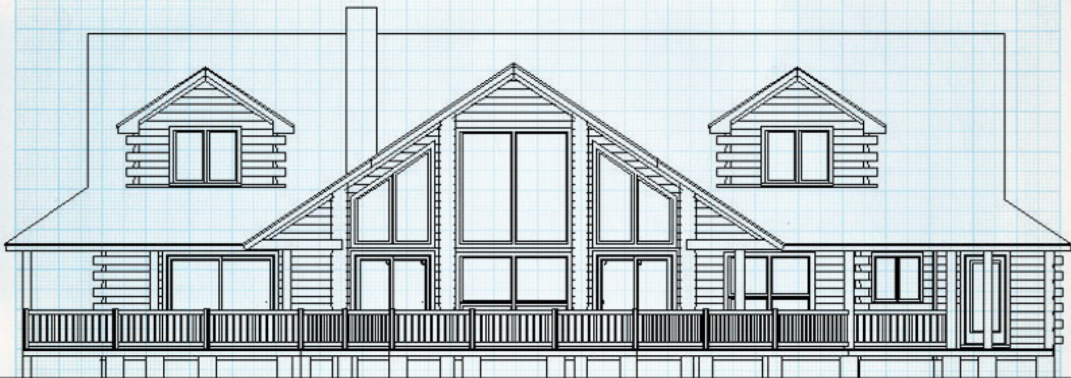
REAR ELEVATION
