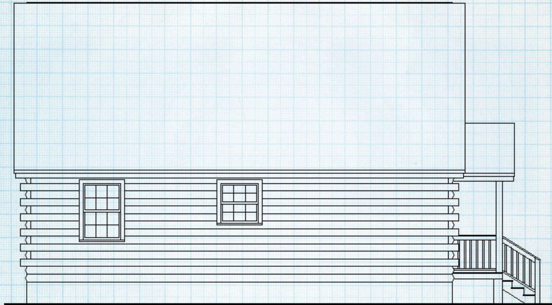
REAR ELEVATION
