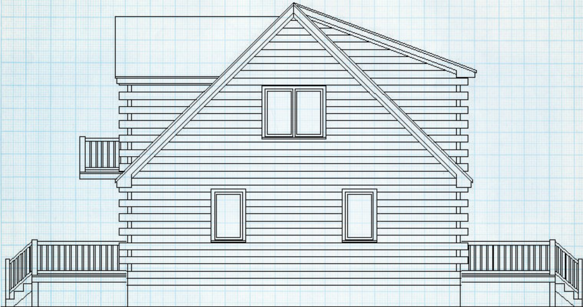
REAR ELEVATION
