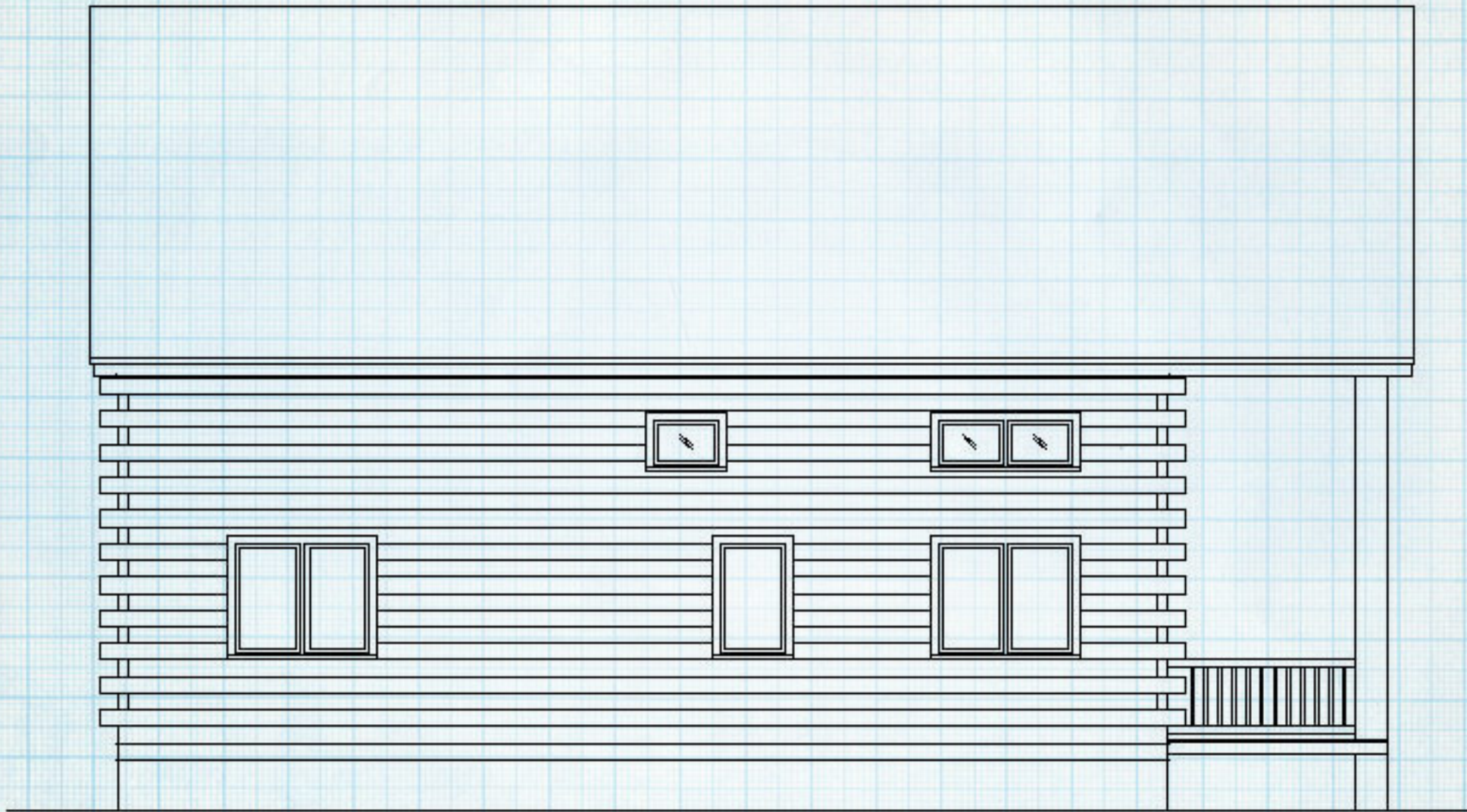
LEFT ELEVATION
