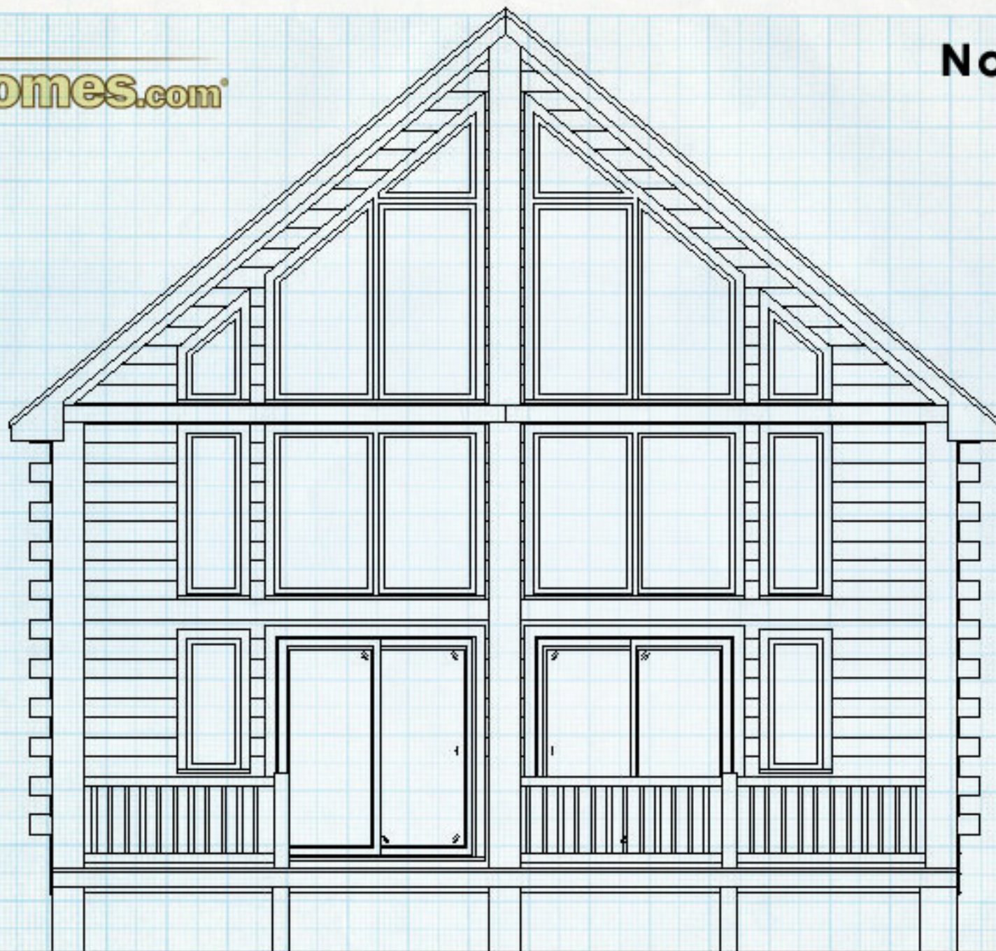
FRONT ELEVATION
